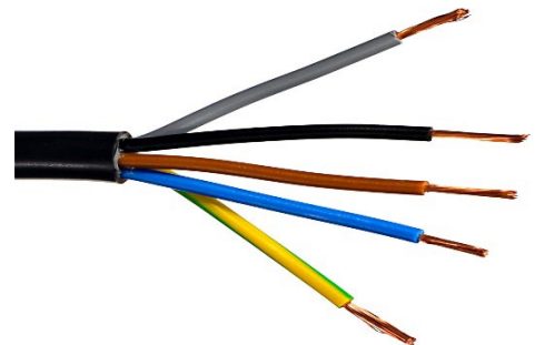
5x1,5mm 2
